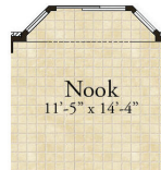
Nook Bay
