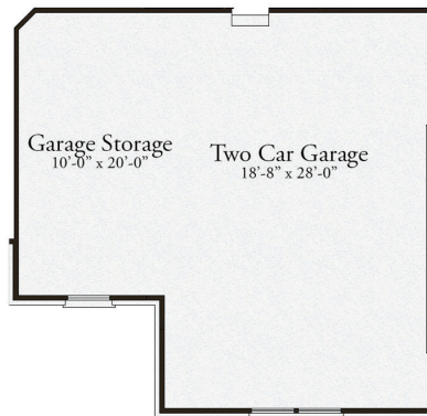
e-Entry Garage with 6' Extension
